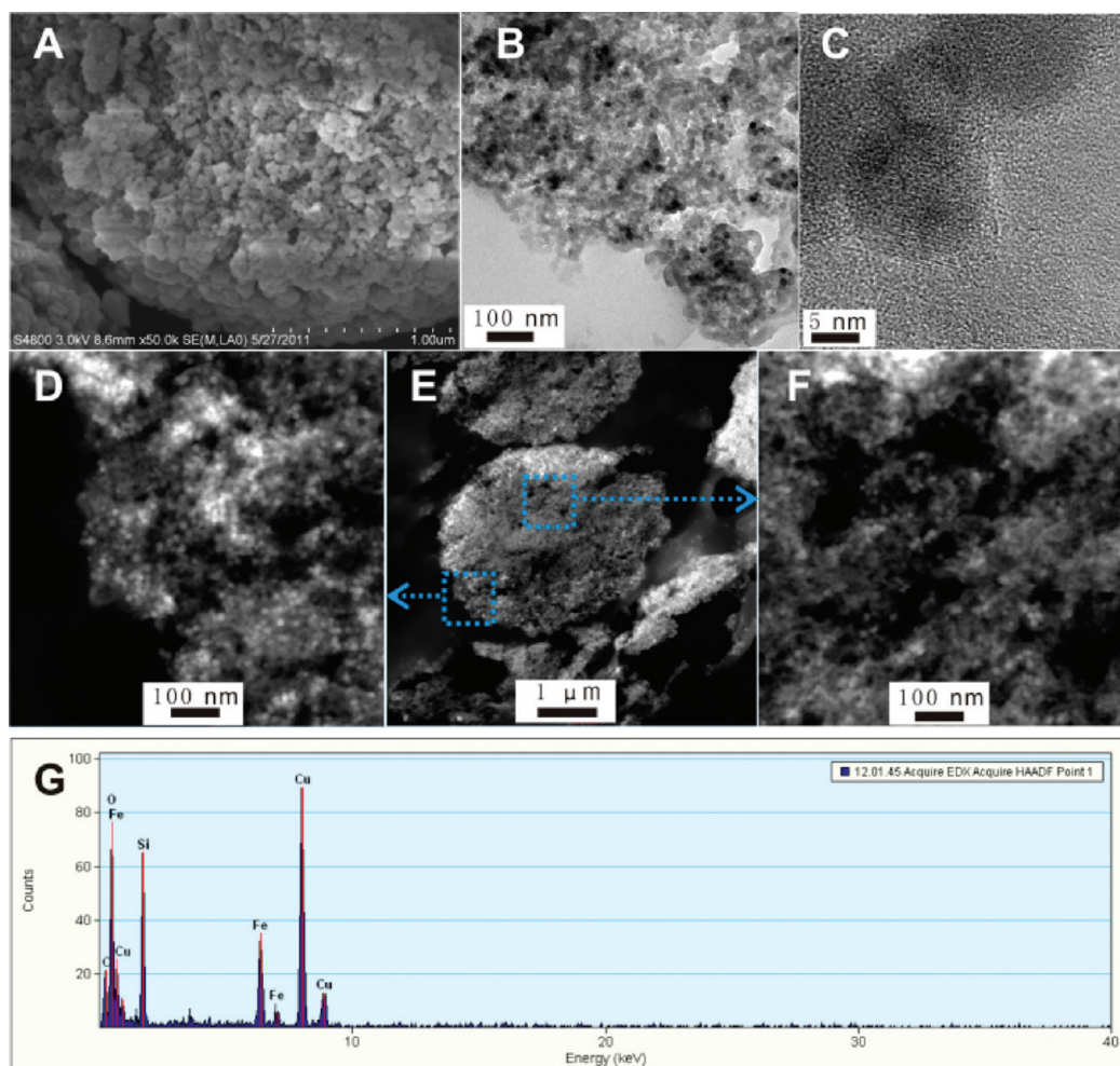
Figure 3. (A) SEM image of the inner structure of \gamma -Fe 2 O 3 /SiO 2 microspheres. (B–C) TEM image of the crashed \gamma -Fe 2 O 3 / SiO 2 microspheres. (D–F) STEM images of \gamma -Fe 2 O 3 /SiO 2 microspheres. (G) EDX map \gamma -Fe 2 O 3 /SiO 2 microspheres.
