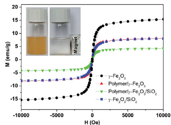
Figure 5. Magnetic hysteresis curves of \gamma-Fe_2O_3 , \gamma-Fe_2O_3 /polymer, \gamma-Fe_2O_3 /polymer/ SiO_2 , and \gamma-Fe_2O_3/SiO_2 microspheres. The inset is a photograph of \gamma-Fe_2O_3/SiO_2 microspheres under external magnetic field.
