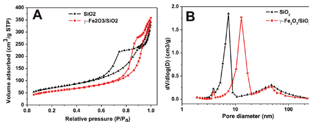
Figure 4. N_2 adsorption/desorption isotherms and pore size distributions of sample SiO_2 and \gamma-Fe_2O_3/SiO_2 microspheres.
